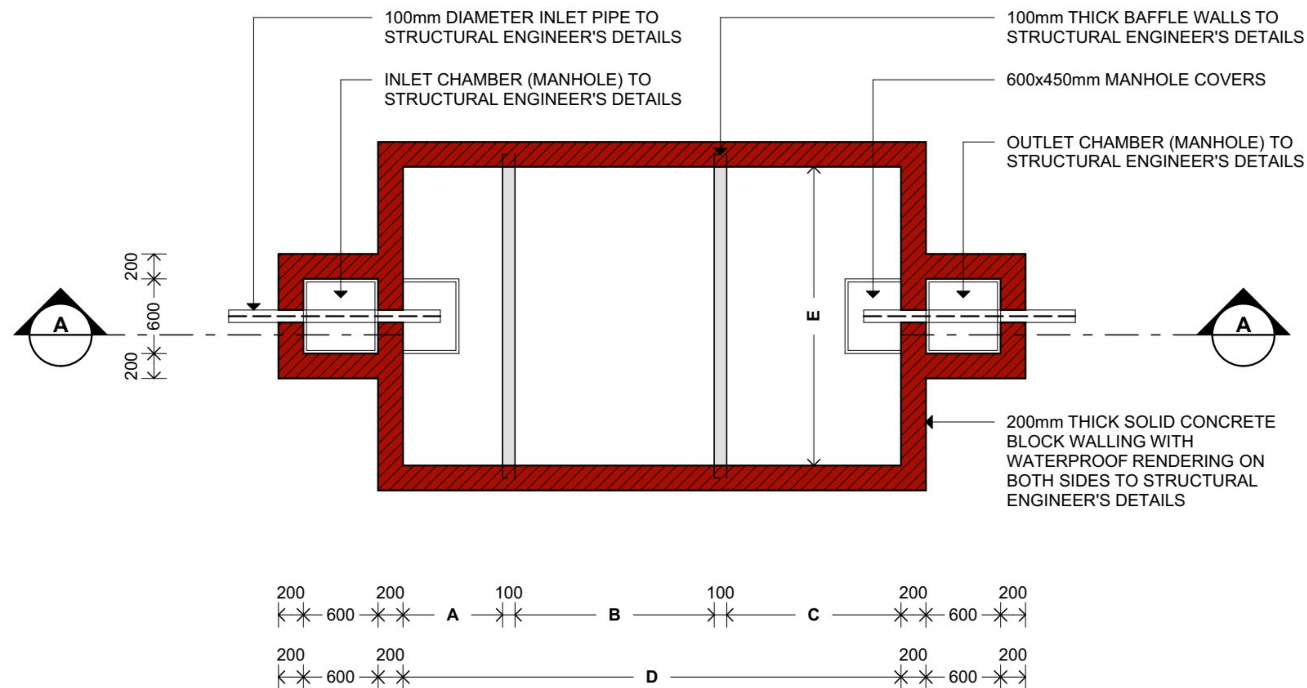
SEPTIC TANK PLAN SCALE 1:50
