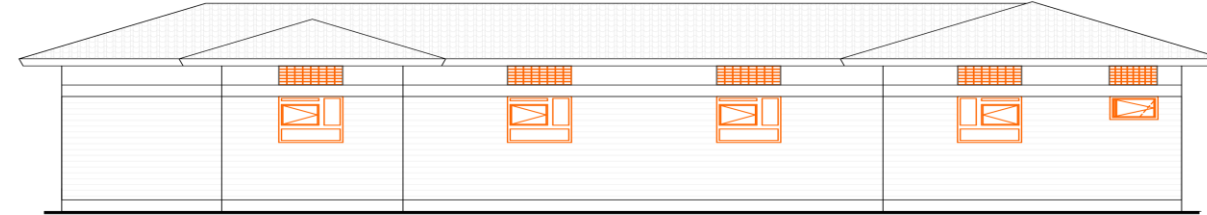
FRONT ELEVATION
