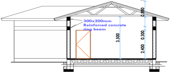
SECTION S-01
