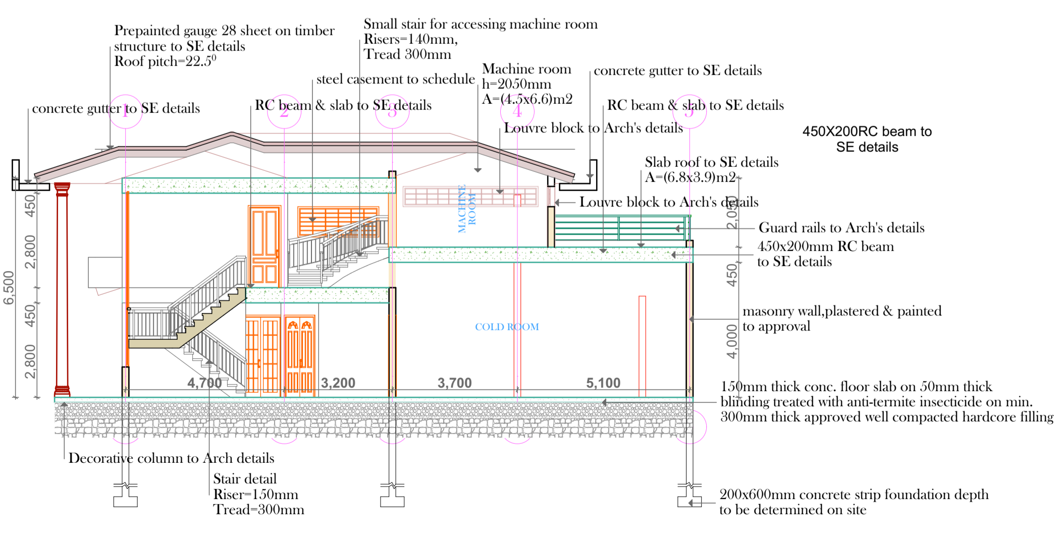
SECTION X-X
