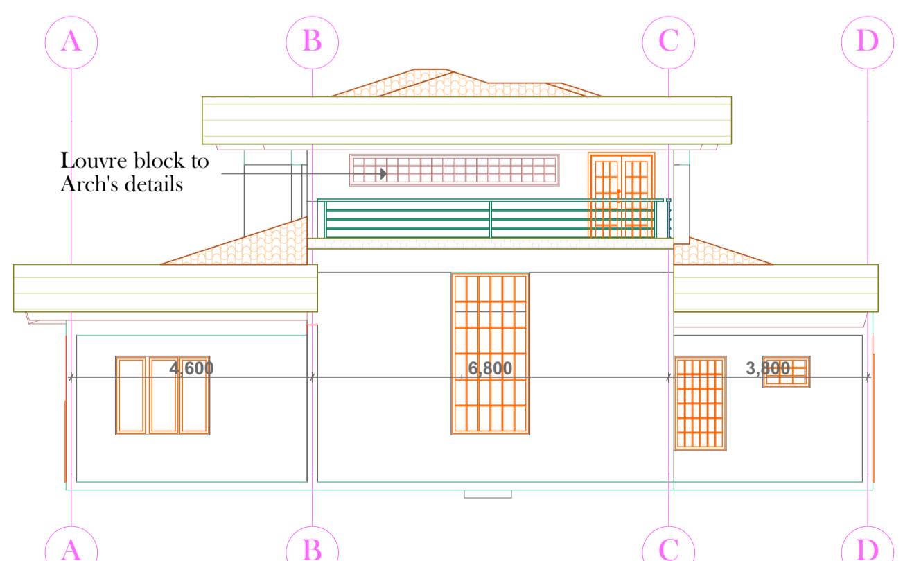
ELEVATION 03
