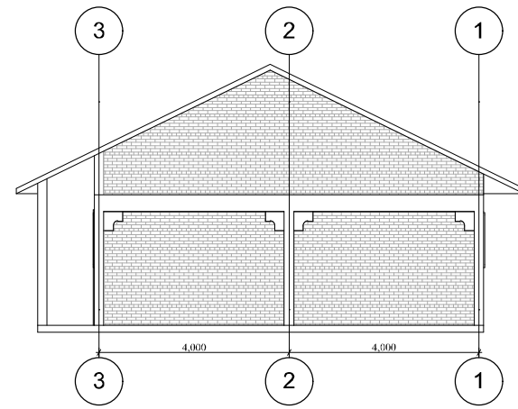
SIDE ELEVATION 01
