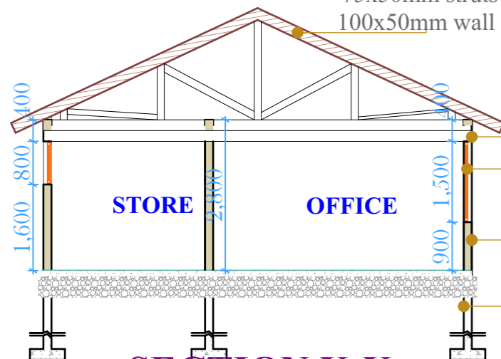
SECTION X-X
