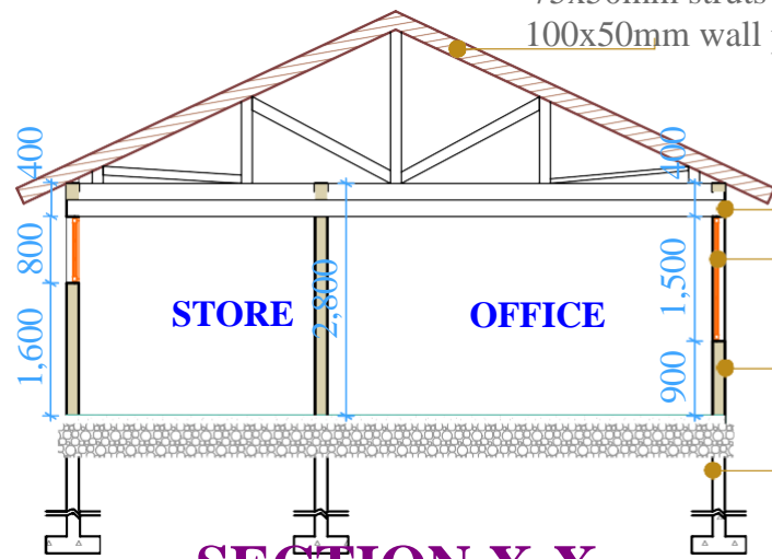
SECTION X-X
