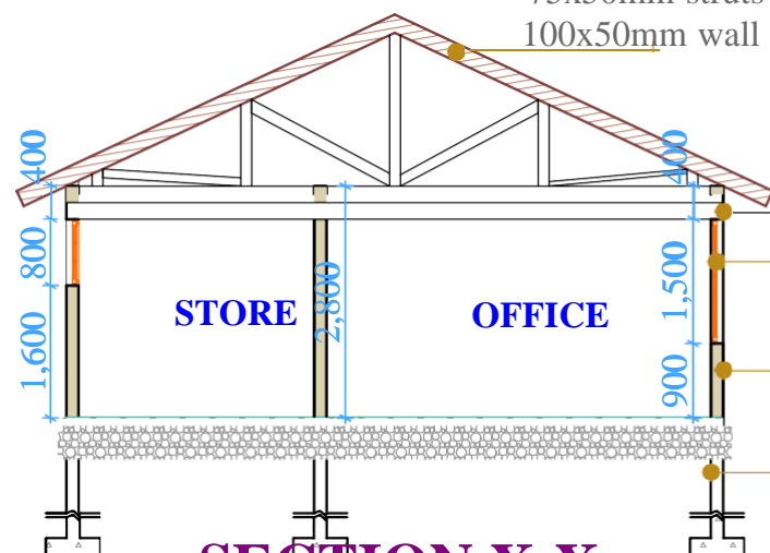
SECTION X-X
