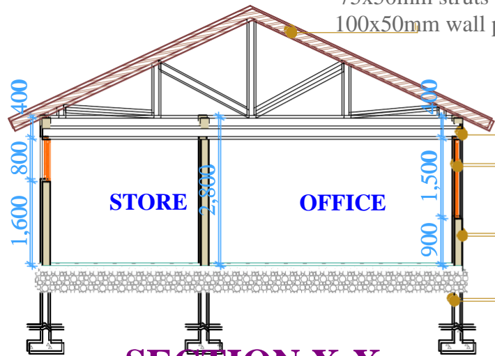
SECTION X-X
