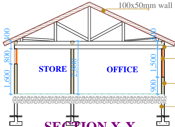
SECTION X-X
